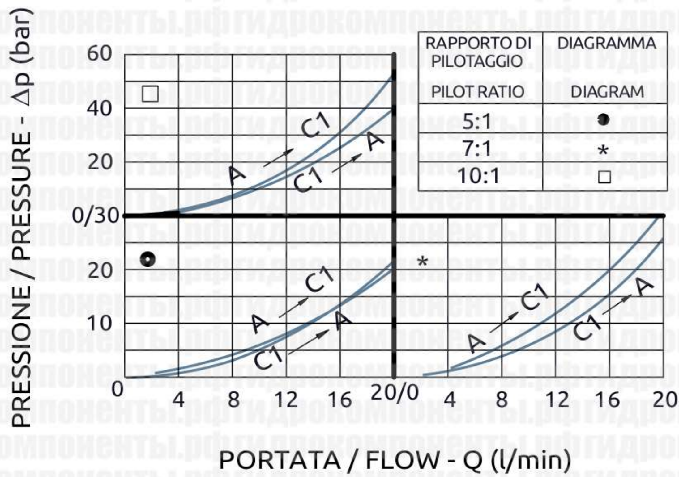
CURVE CARATTERISTICHE PERFORMANCE CURVES
